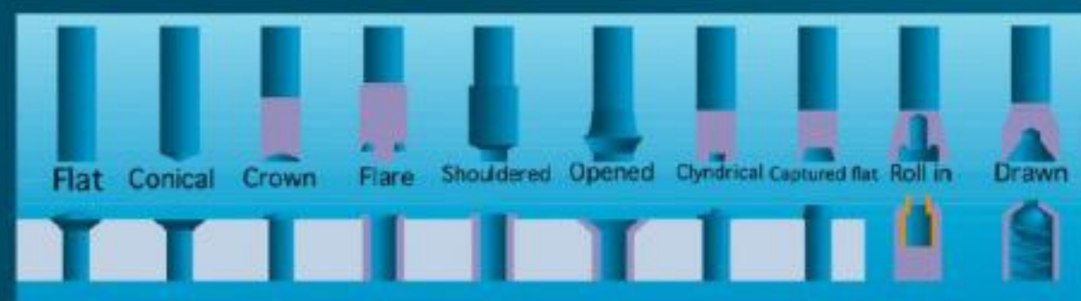
LONG REACH ORBITAL HEADS (HL)
